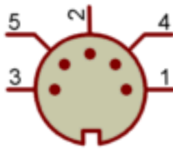
Female DIN plug Soldering side
